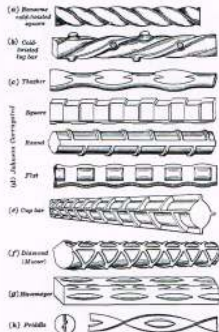
A series of deformed bars.
