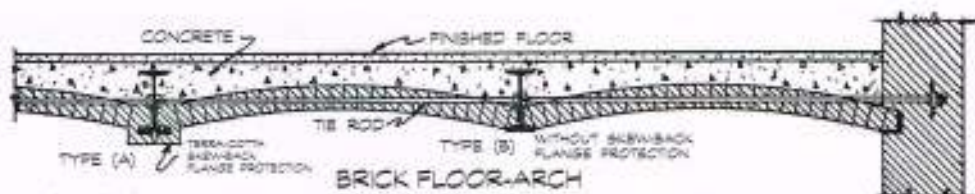
Brick Arch Floor.
